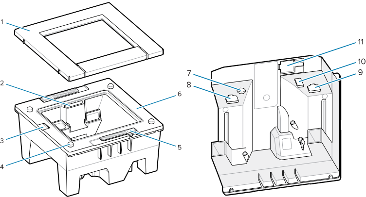
Figure 4 SP7208-H Scanner
