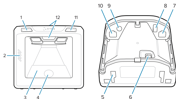
Figure 2 SP7208-V Scanner
