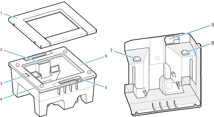
Figure 3 SP7201-H Scanner
